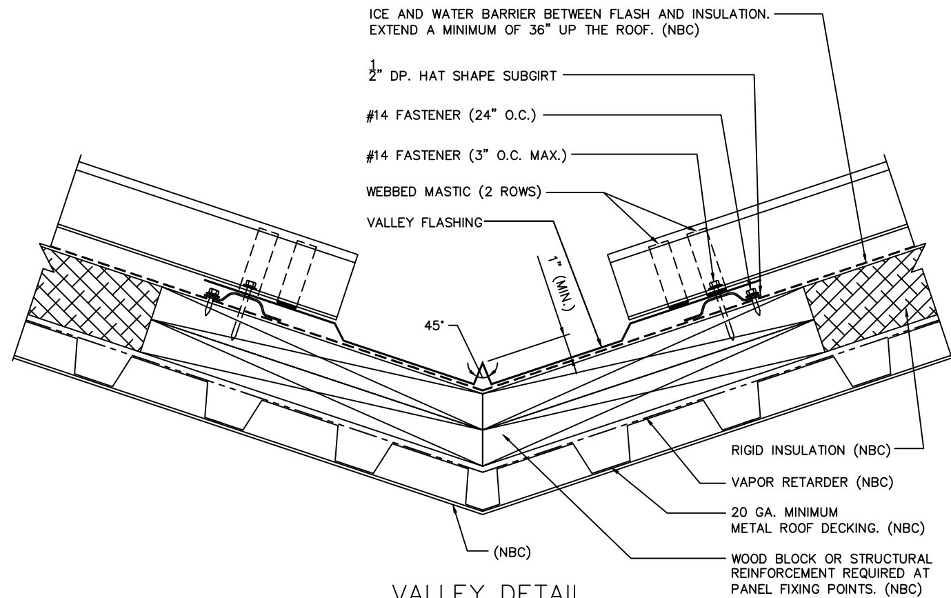
VALLEY DETAIL
