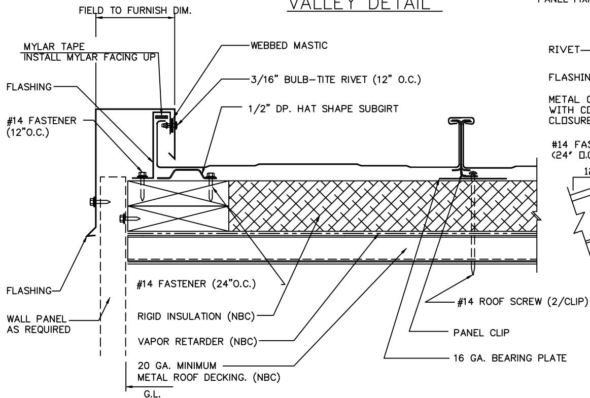
BOX GABLE DETAIL
