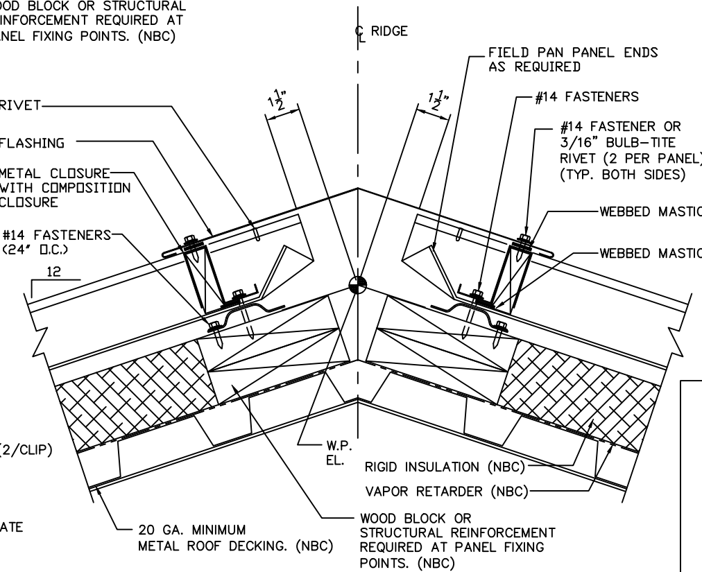
RIDGE DETAIL
