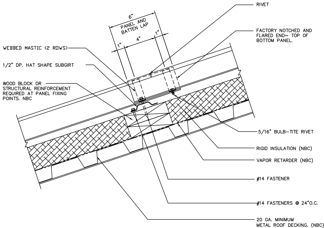
PANEL ENDLAP DETAIL
