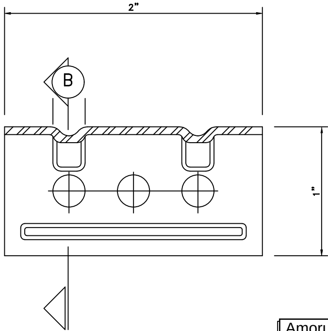
SECTION A
