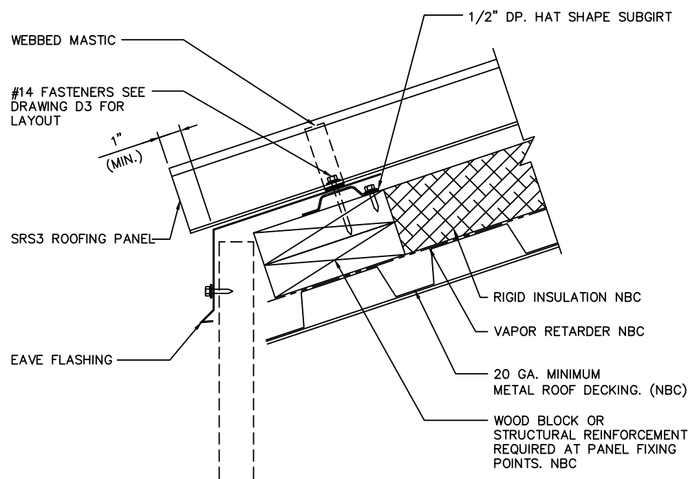
EAVE DETAIL
