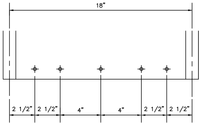
SRS3-1.5 FIXED END FASTENER SPACING
