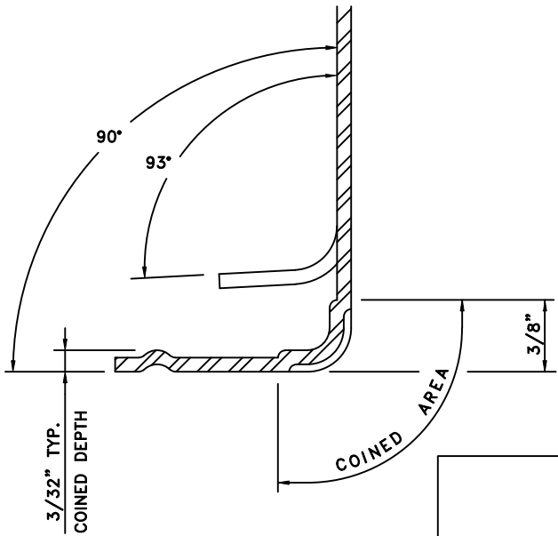
SECTION B
